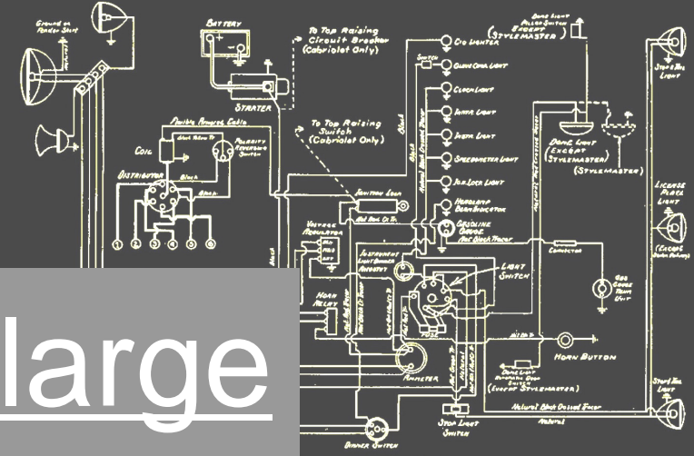
1940 Chevrolet-Passenger Car Wiring Diagram
